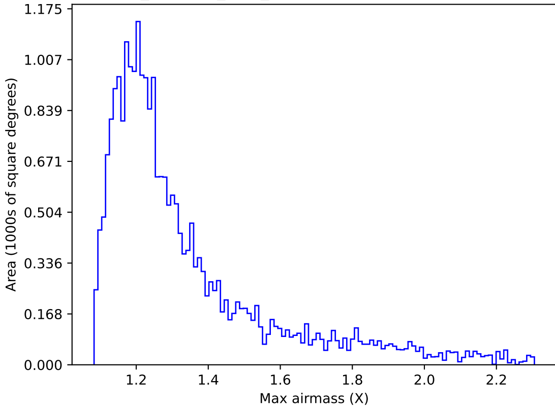
retro_baseline_v2.0_10yrs Yr 1 g band: Max airmass
