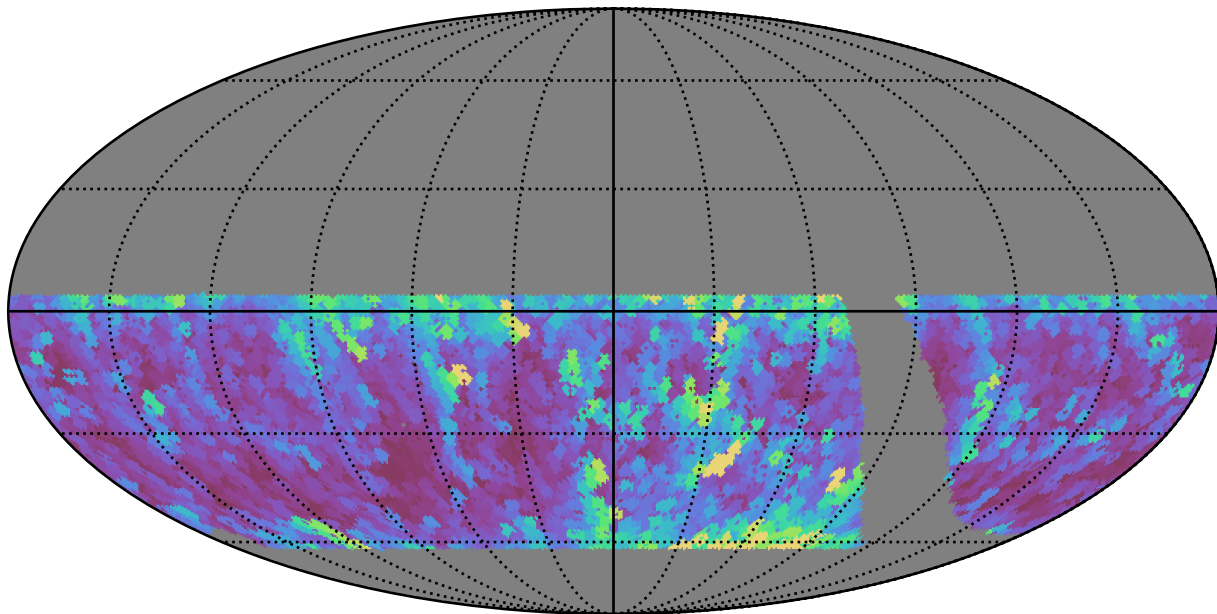
retro_baseline_v2.0_10yrs WFD z band: Max airmass
