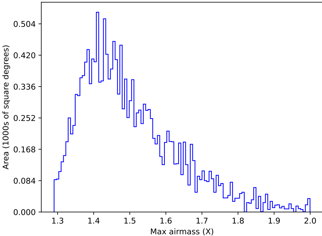
retro_baseline_v2.0_10yrs WFD z band: Max airmass
