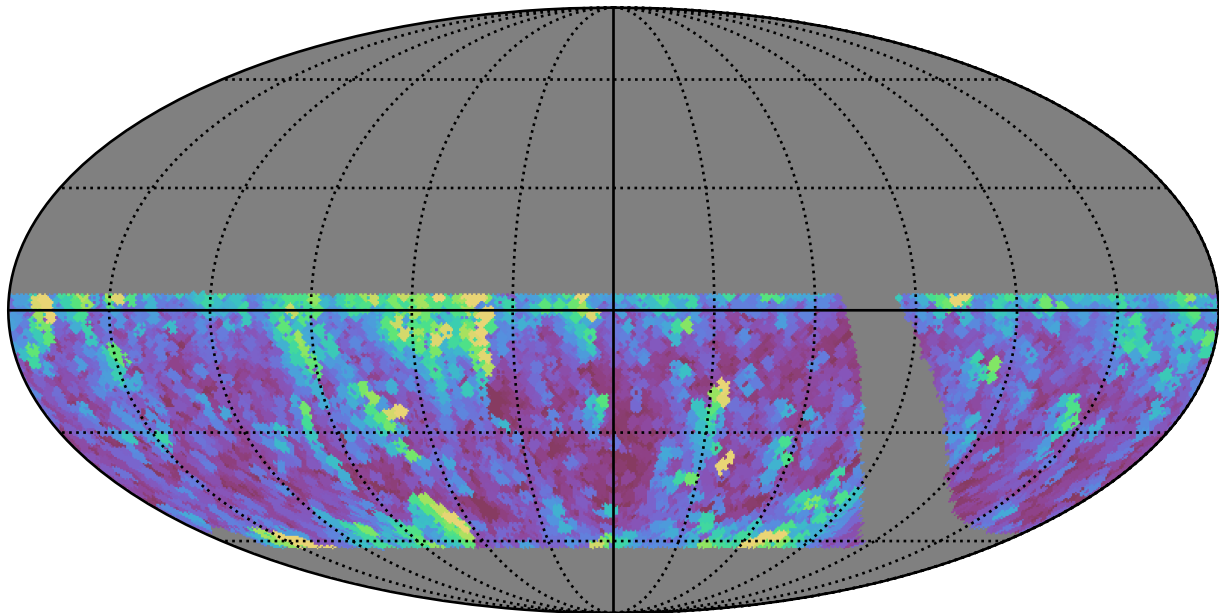
retro_baseline_v2.0_10yrs WFD y band: Max airmass
