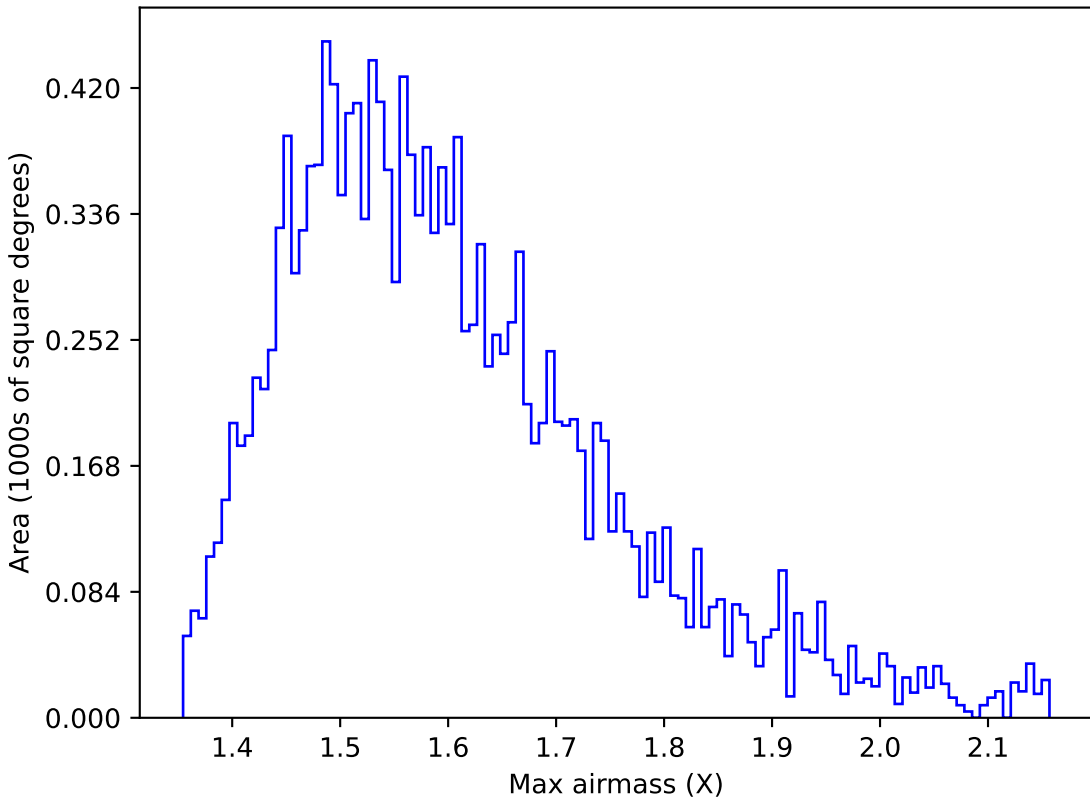
retro_baseline_v2.0_10yrs WFD y band: Max airmass
