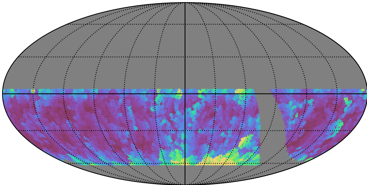
retro_baseline_v2.0_10yrs WFD u band: Max airmass
