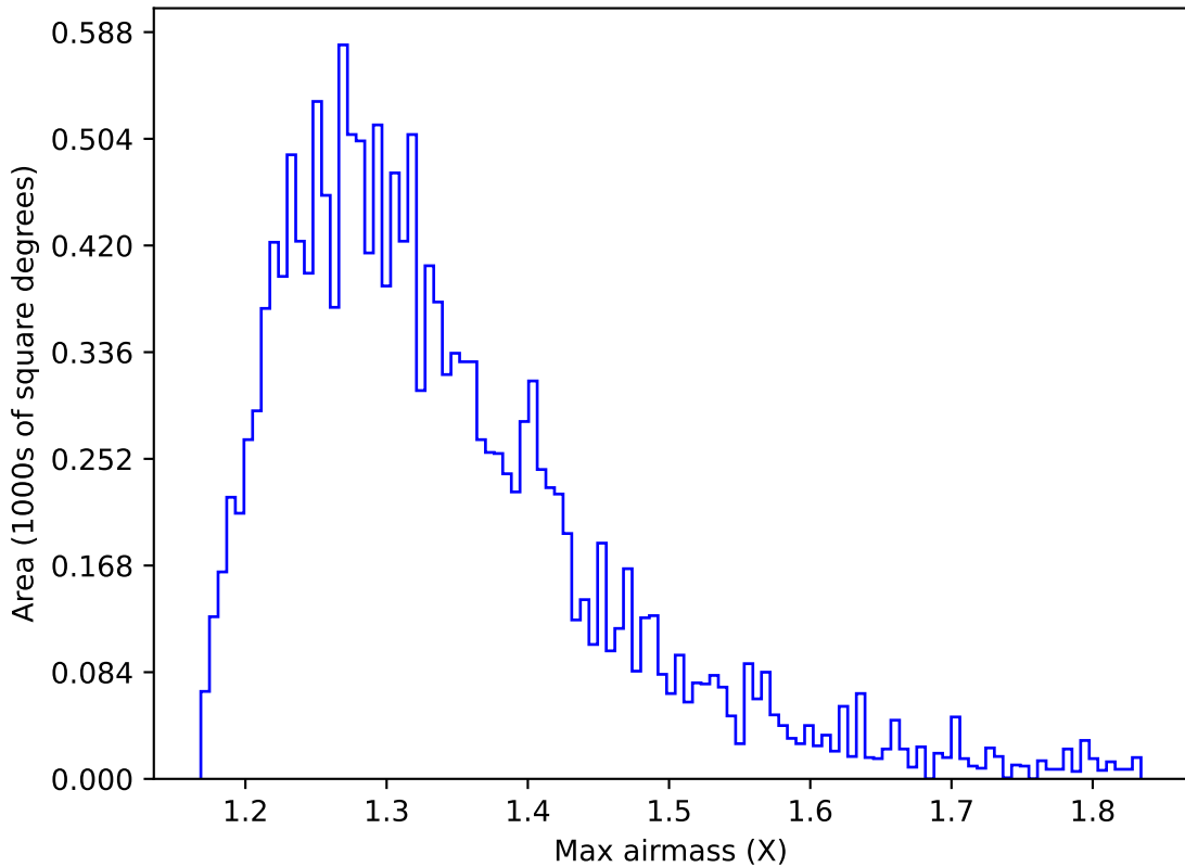
retro_baseline_v2.0_10yrs WFD u band: Max airmass
