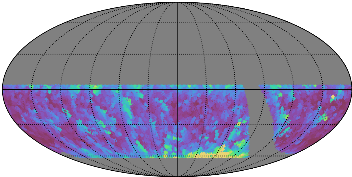
retro_baseline_v2.0_10yrs WFD r band: Max airmass
