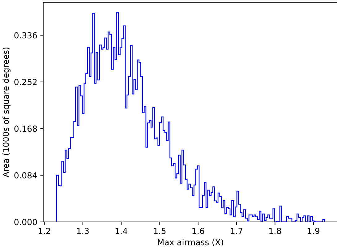
retro_baseline_v2.0_10yrs WFD r band: Max airmass
