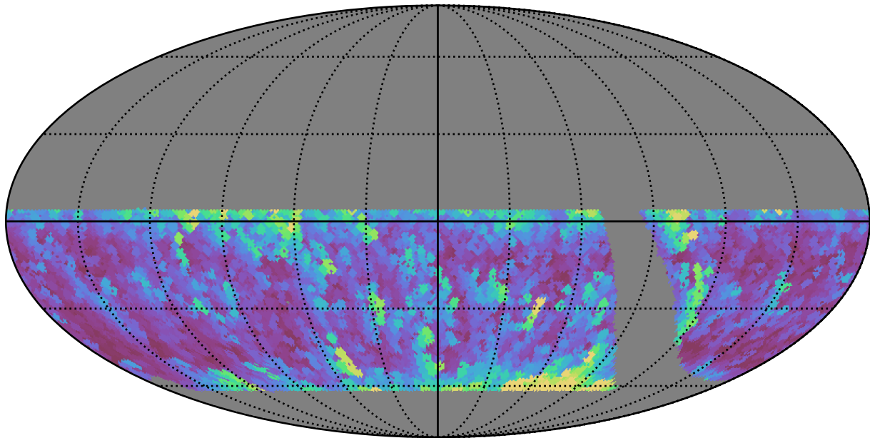
retro_baseline_v2.0_10yrs WFD i band: Max airmass
