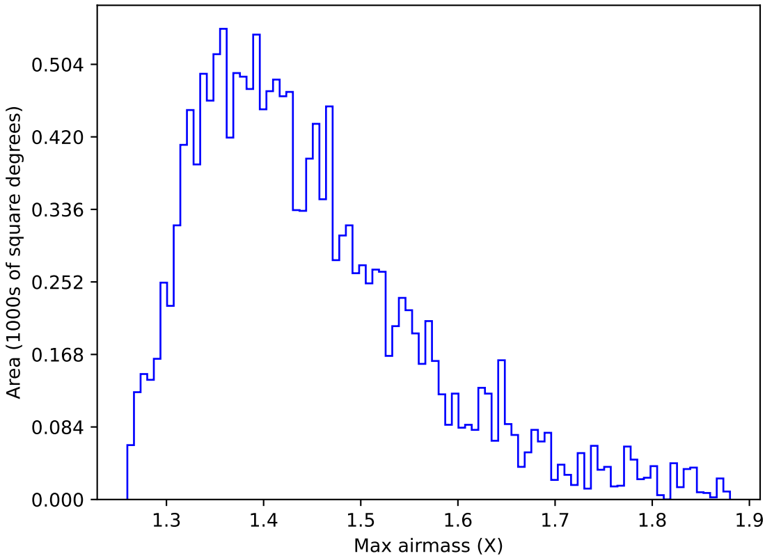
retro_baseline_v2.0_10yrs WFD i band: Max airmass
