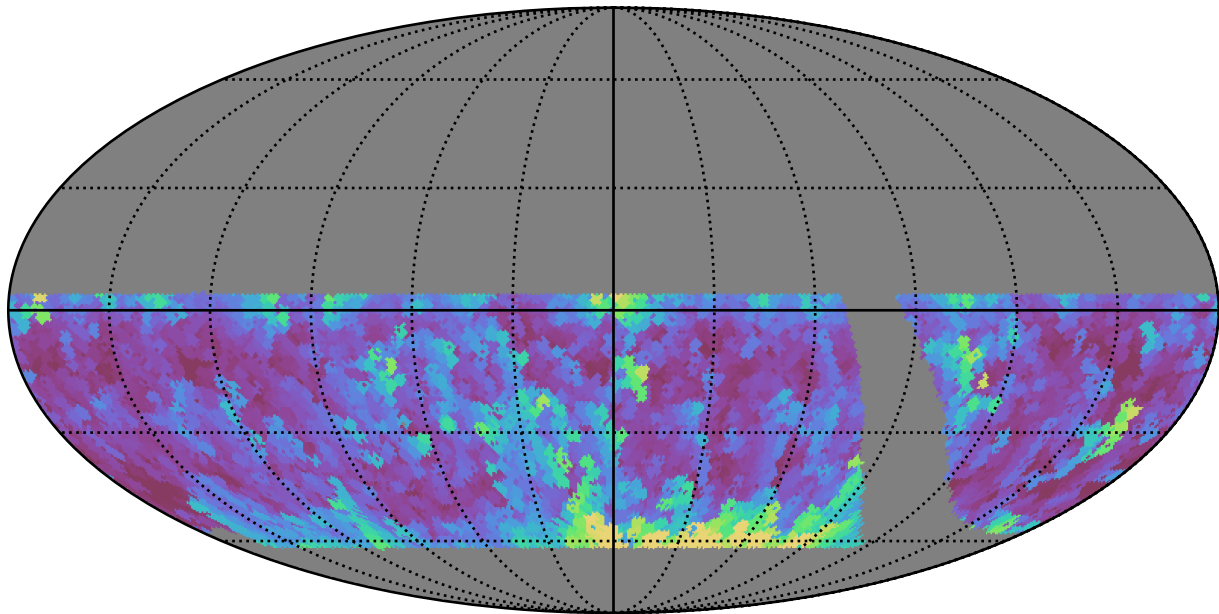
retro_baseline_v2.0_10yrs WFD g band: Max airmass
