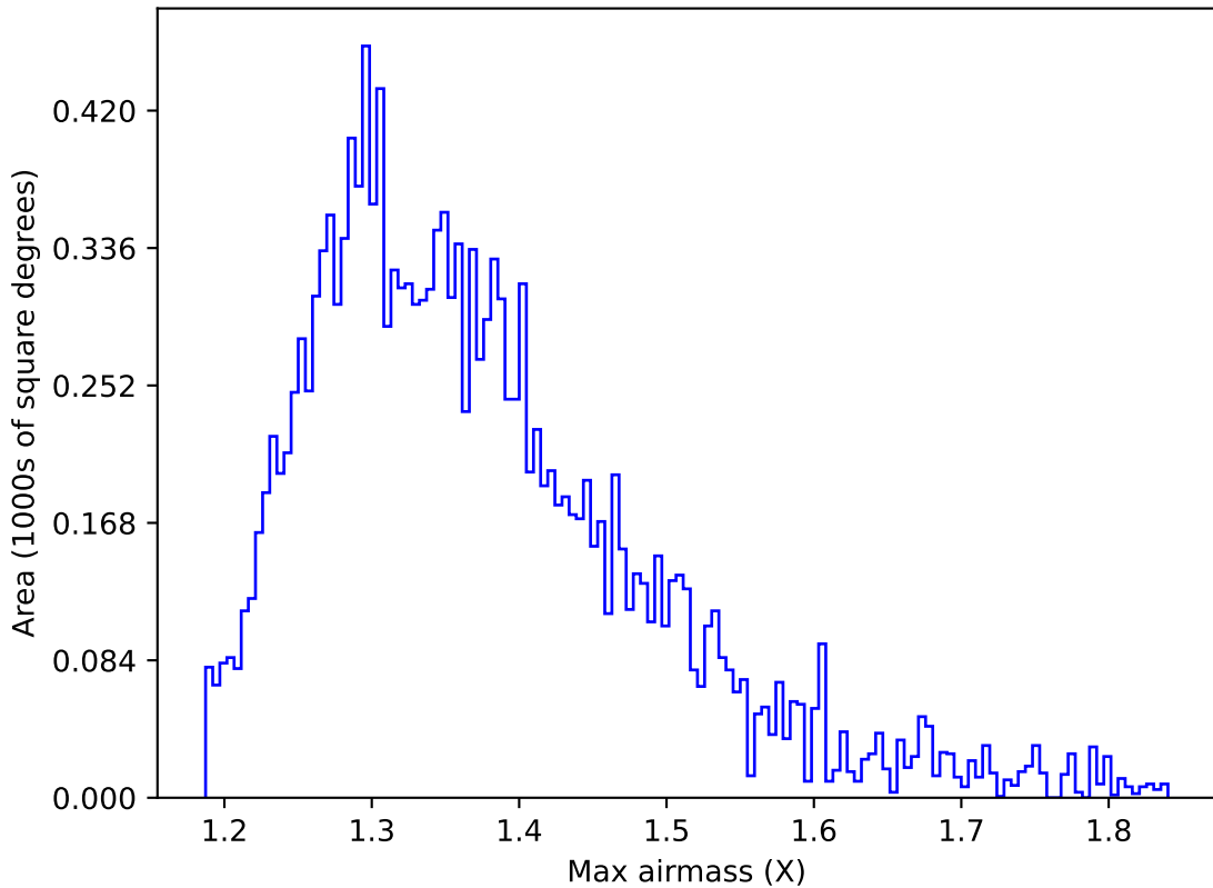
retro_baseline_v2.0_10yrs WFD g band: Max airmass
