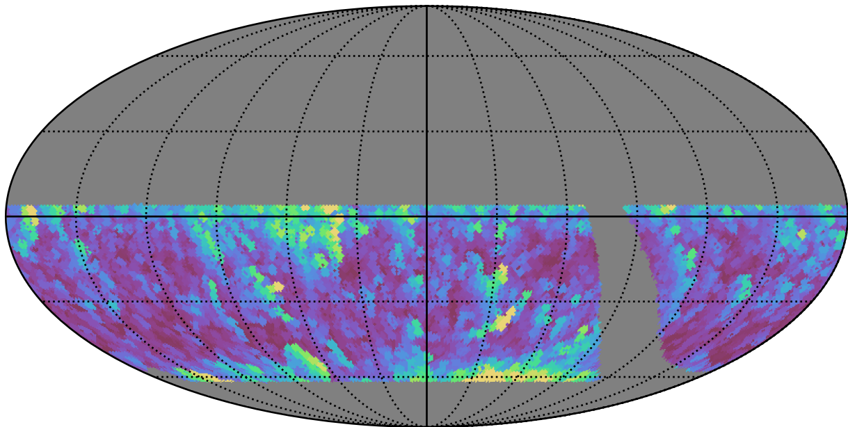
retro_baseline_v2.0_10yrs WFD all bands: Max airmass
