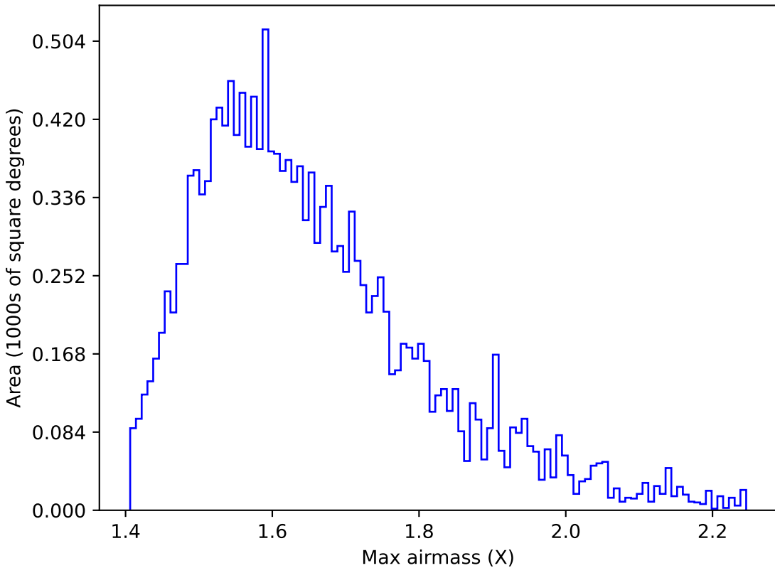
retro_baseline_v2.0_10yrs WFD all bands: Max airmass
