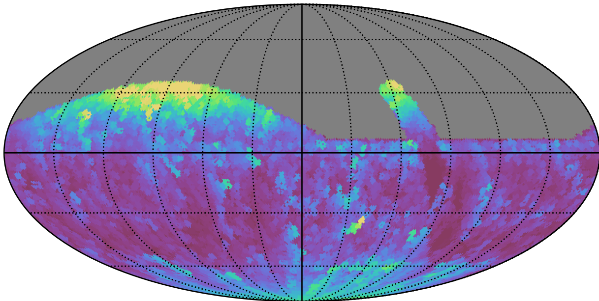
retro_baseline_v2.0_10yrs All sky z band: Max airmass
