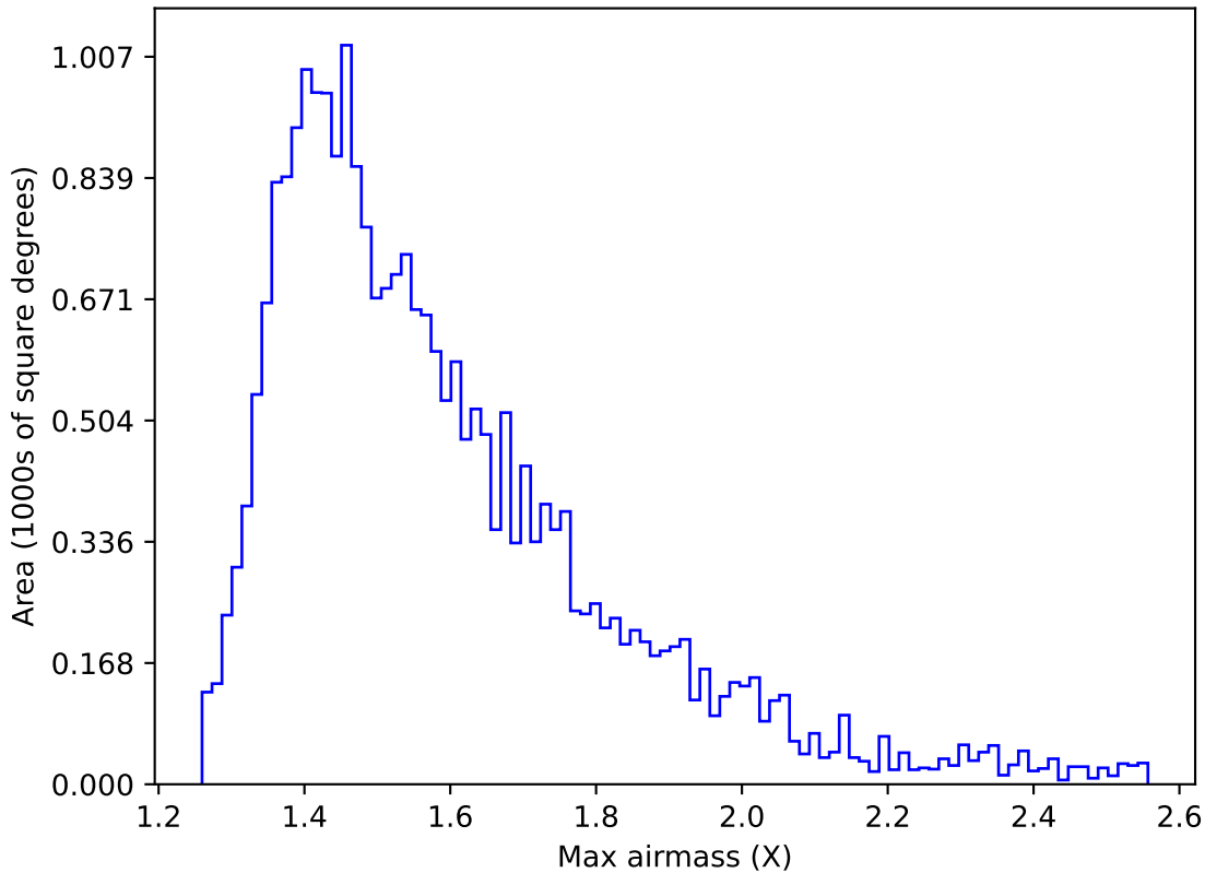
retro_baseline_v2.0_10yrs All sky z band: Max airmass
