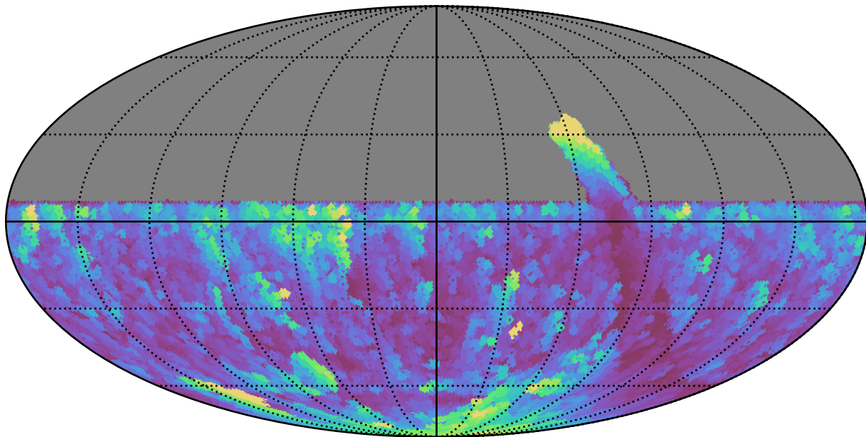
retro_baseline_v2.0_10yrs All sky y band: Max airmass
