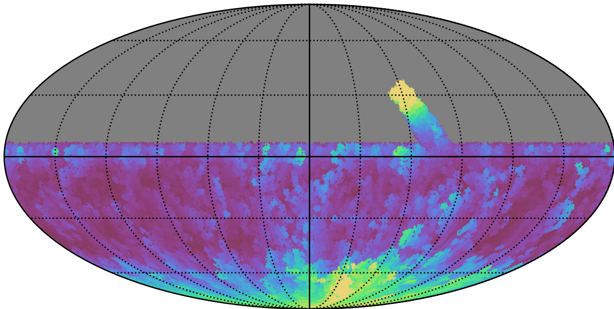
retro_baseline_v2.0_10yrs All sky u band: Max airmass
