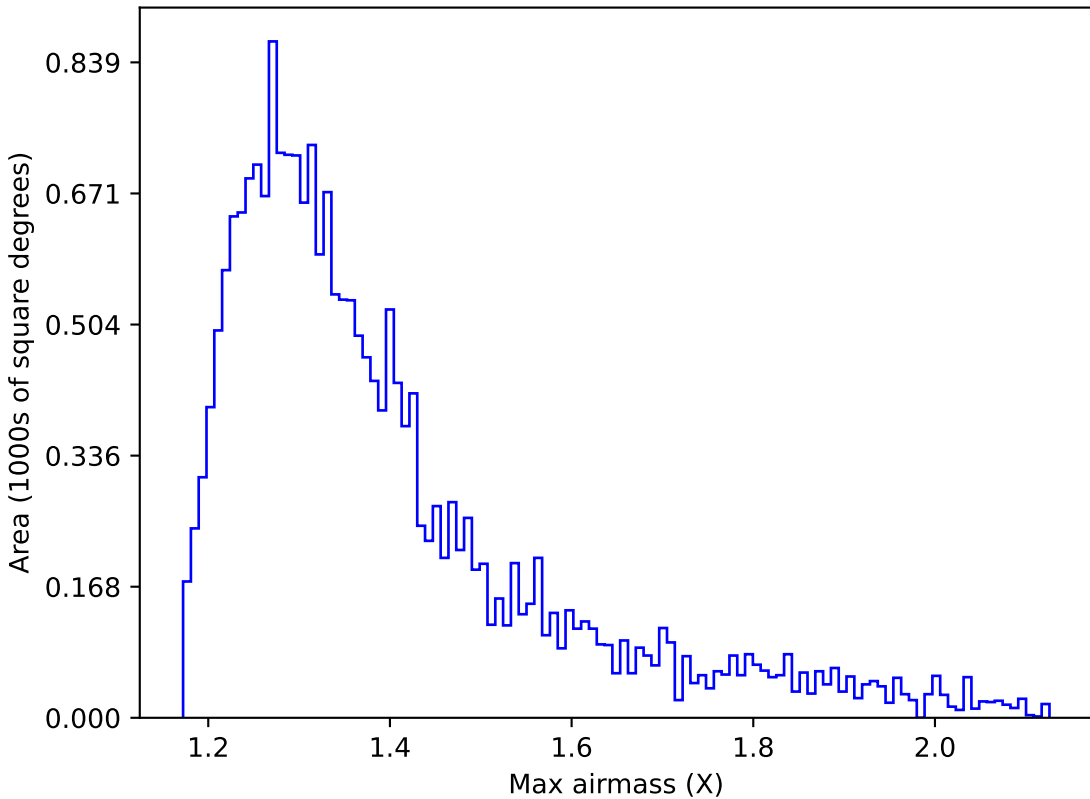
retro_baseline_v2.0_10yrs All sky u band: Max airmass
