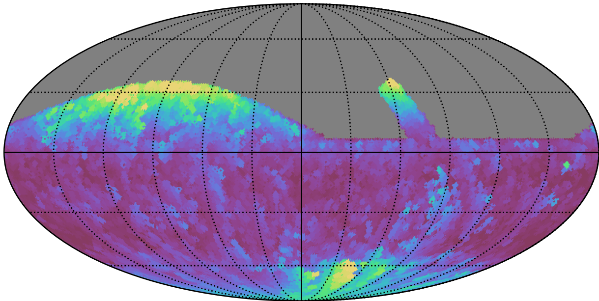
retro_baseline_v2.0_10yrs All sky r band: Max airmass
