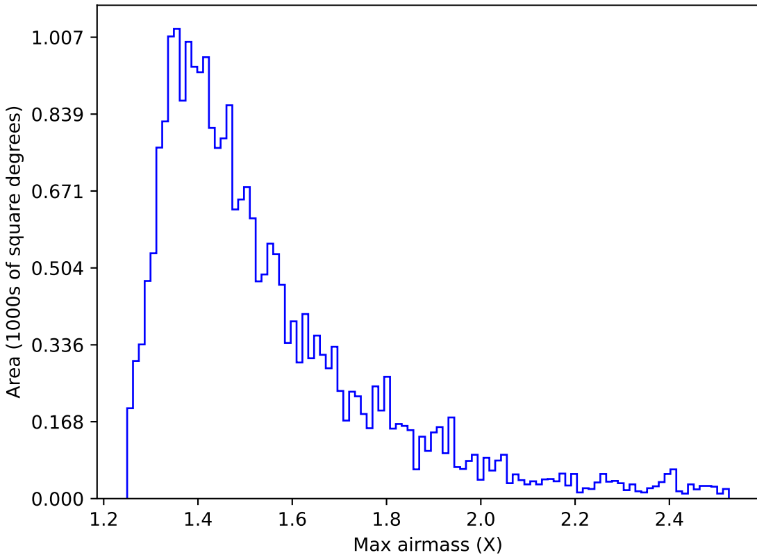
retro_baseline_v2.0_10yrs All sky i band: Max airmass
