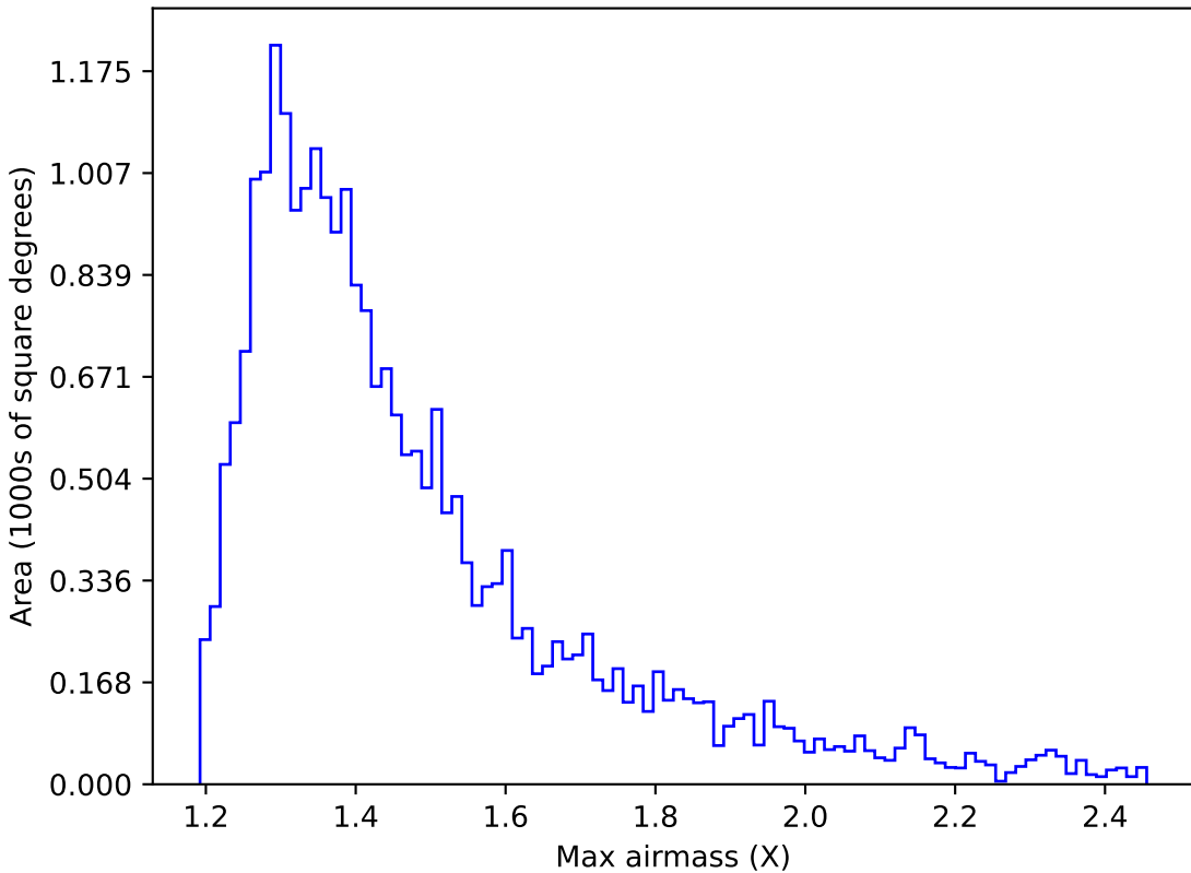
retro_baseline_v2.0_10yrs All sky g band: Max airmass
