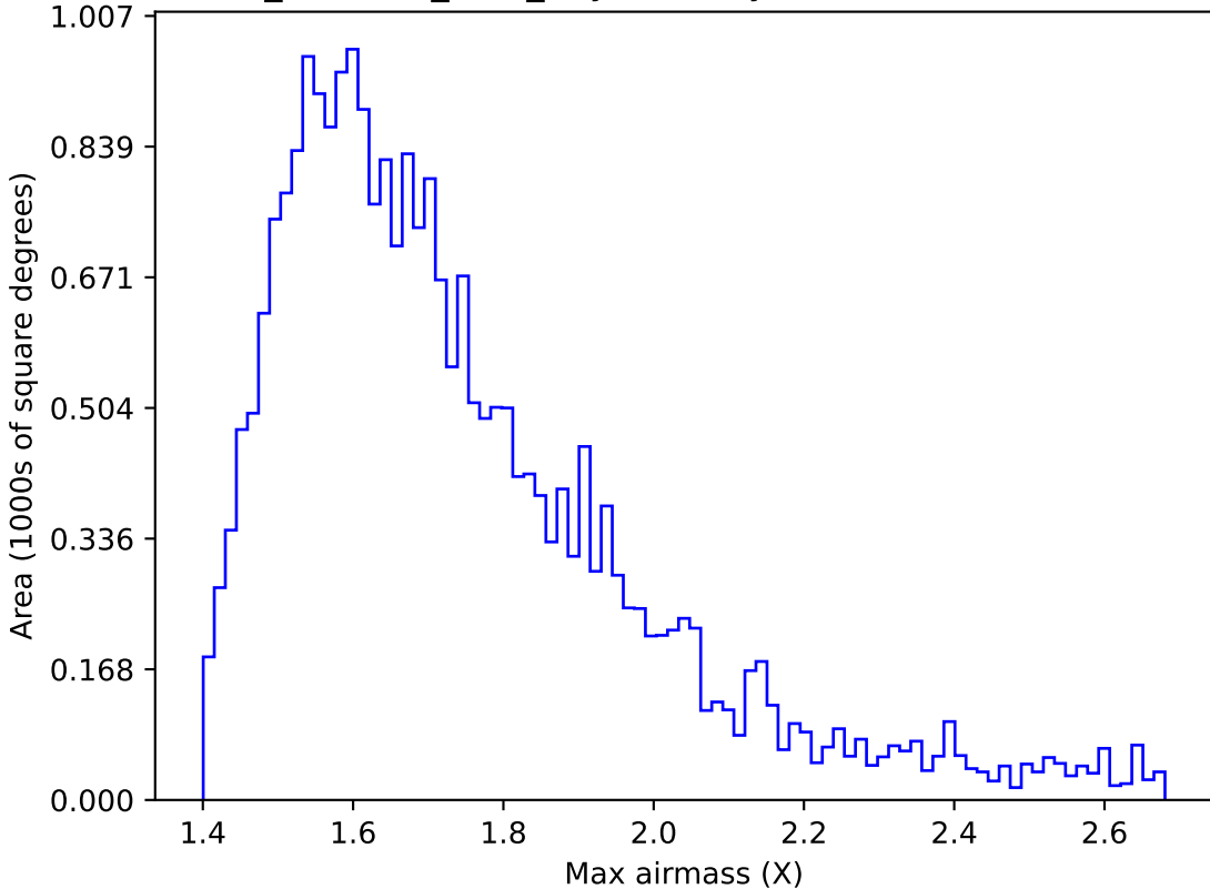
retro_baseline_v2.0_10yrs All sky all bands: Max airmass
