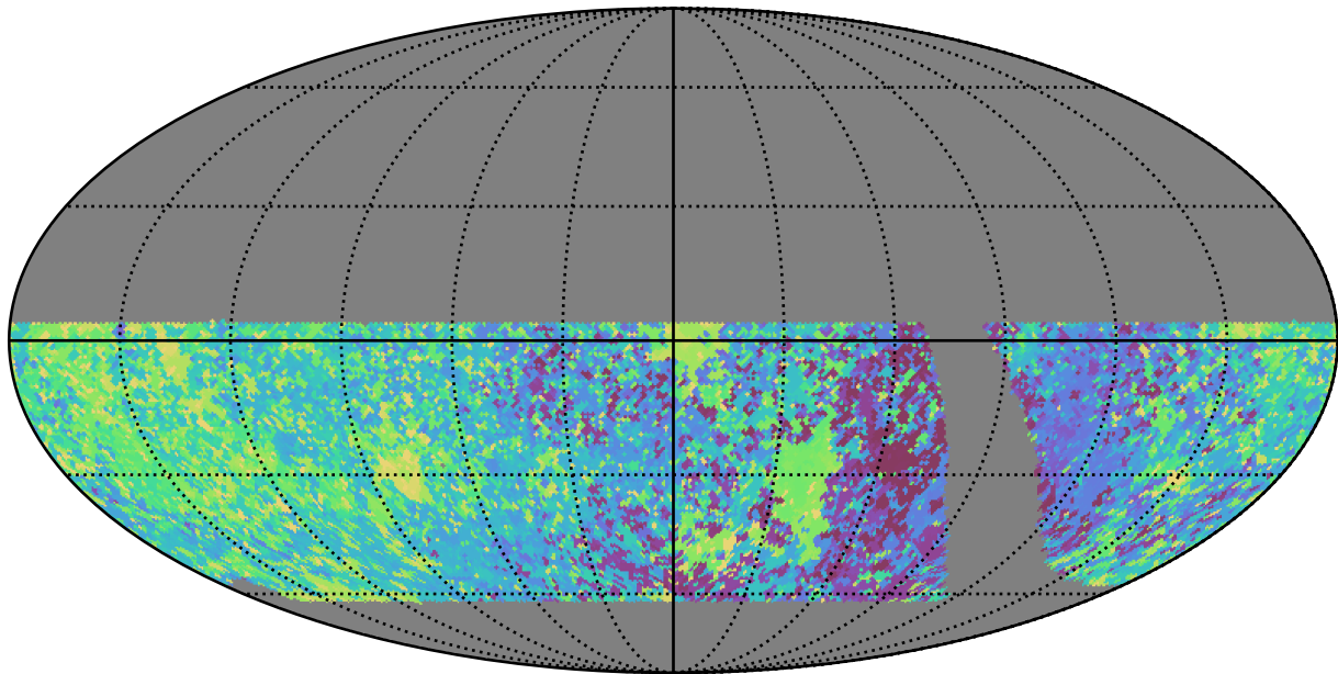
retro_baseline_v2.0_10yrs WFD z band: Max Inter-Night Gap
