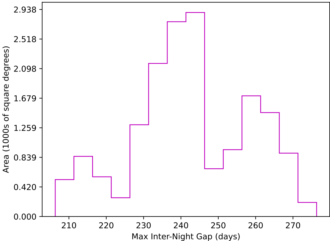
retro_baseline_v2.0_10yrs WFD z band: Max Inter-Night Gap
