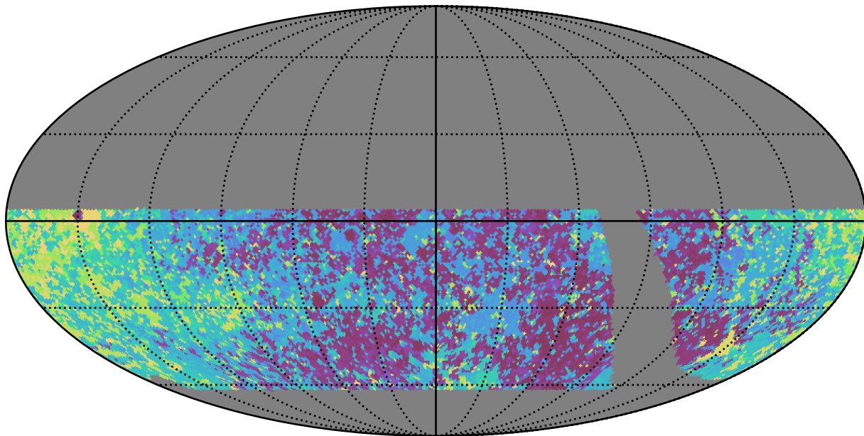
retro_baseline_v2.0_10yrs WFD y band: Max Inter-Night Gap
