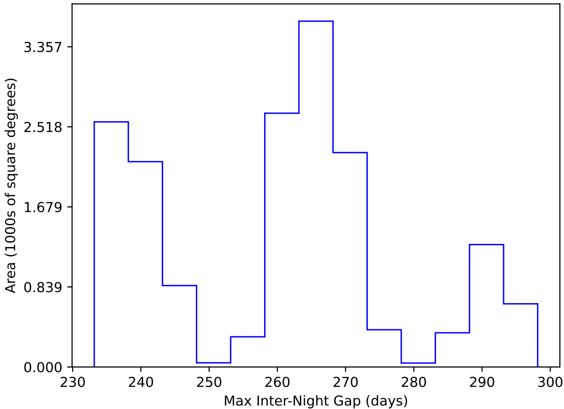
retro_baseline_v2.0_10yrs WFD y band: Max Inter-Night Gap
