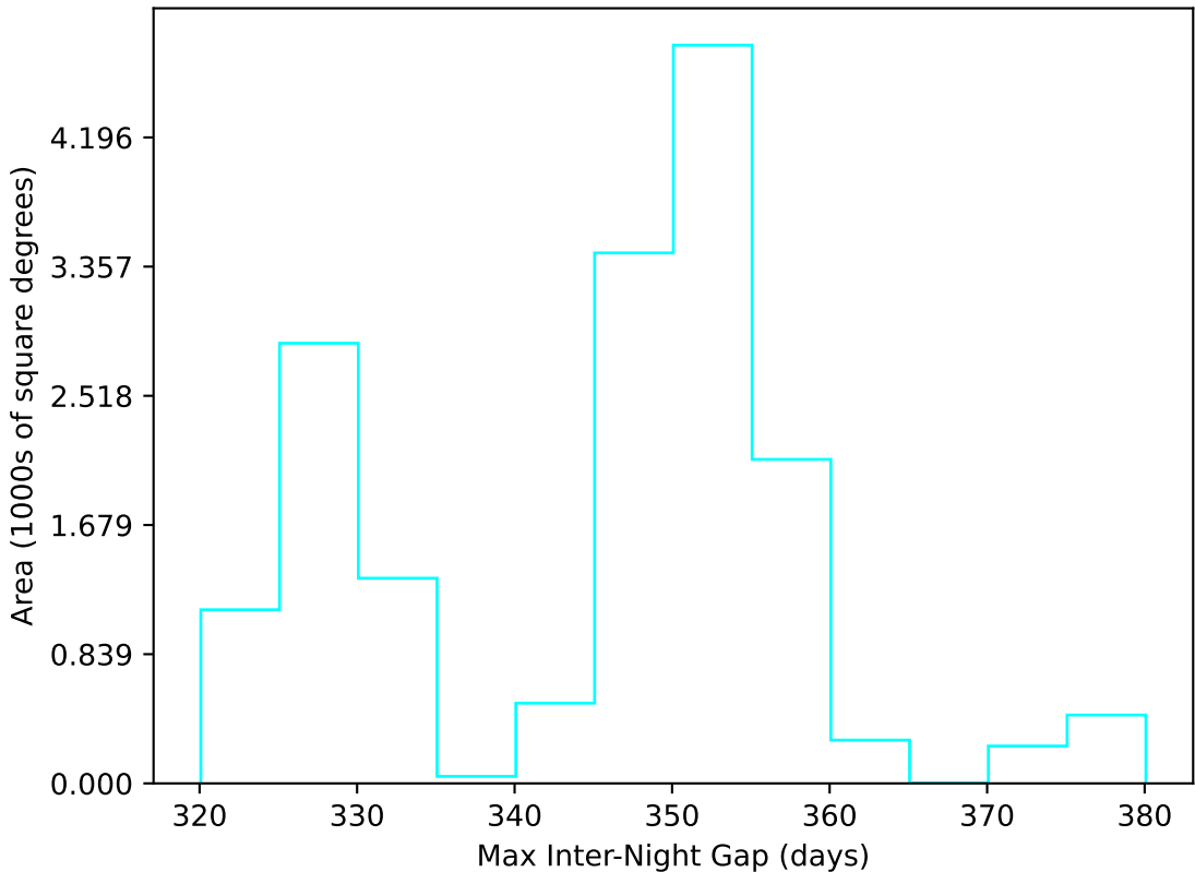
retro_baseline_v2.0_10yrs WFD u band: Max Inter-Night Gap
