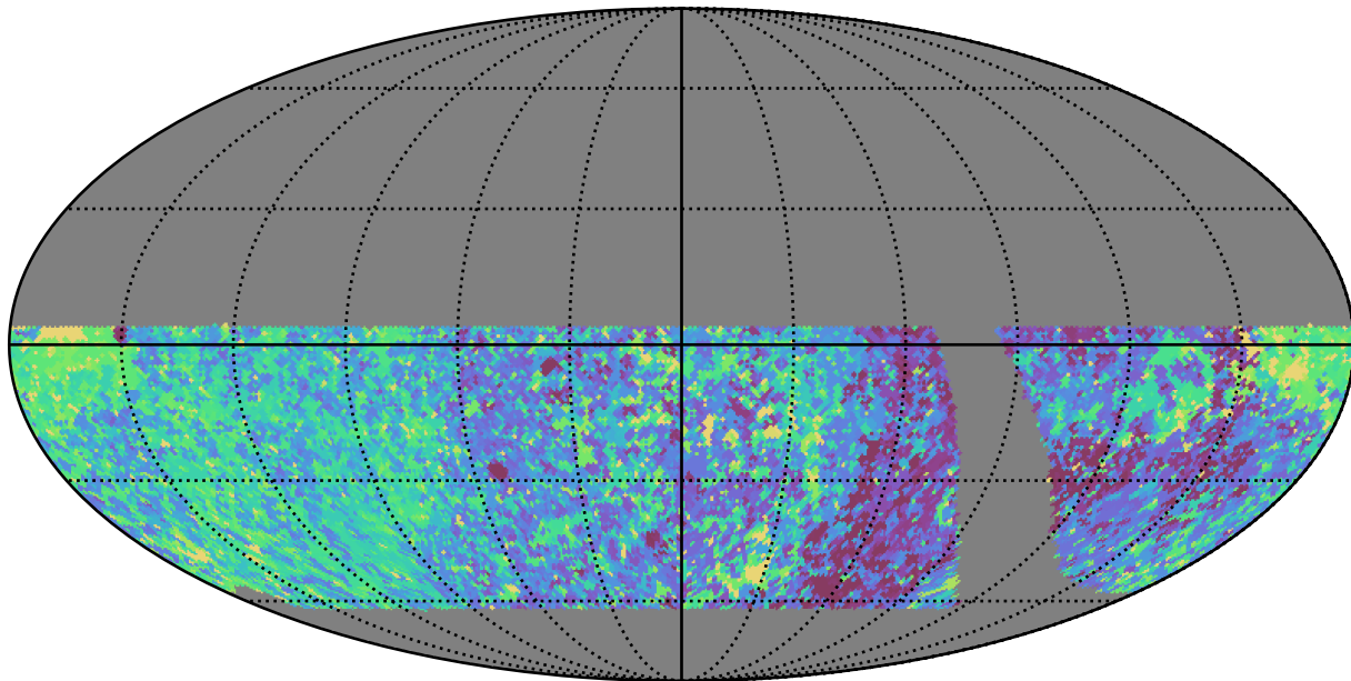
retro_baseline_v2.0_10yrs WFD r band: Max Inter-Night Gap
