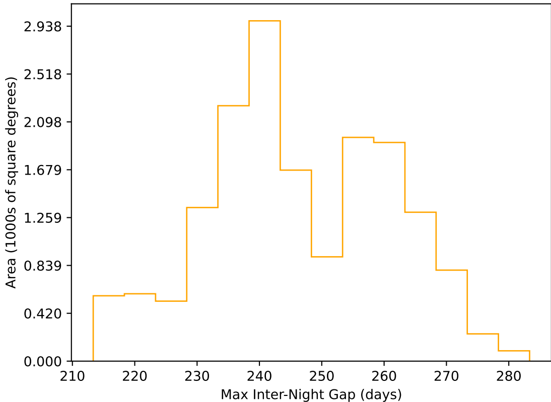
retro_baseline_v2.0_10yrs WFD r band: Max Inter-Night Gap
