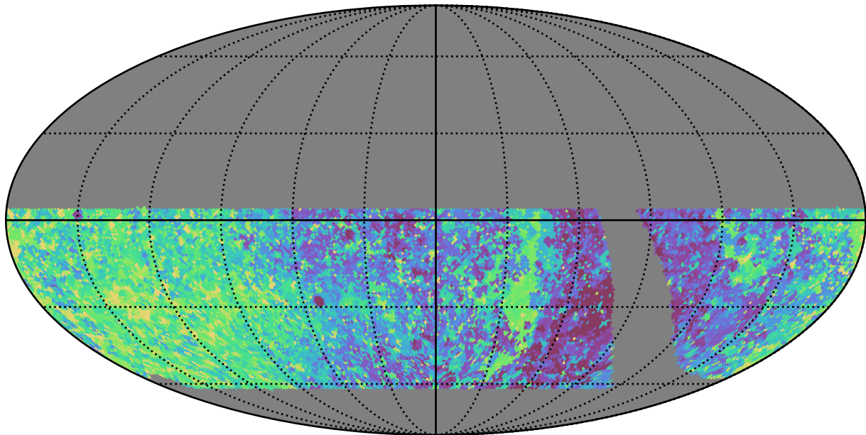
retro_baseline_v2.0_10yrs WFD i band: Max Inter-Night Gap
