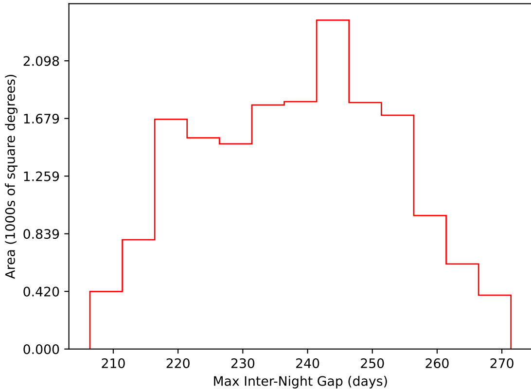
retro_baseline_v2.0_10yrs WFD i band: Max Inter-Night Gap
