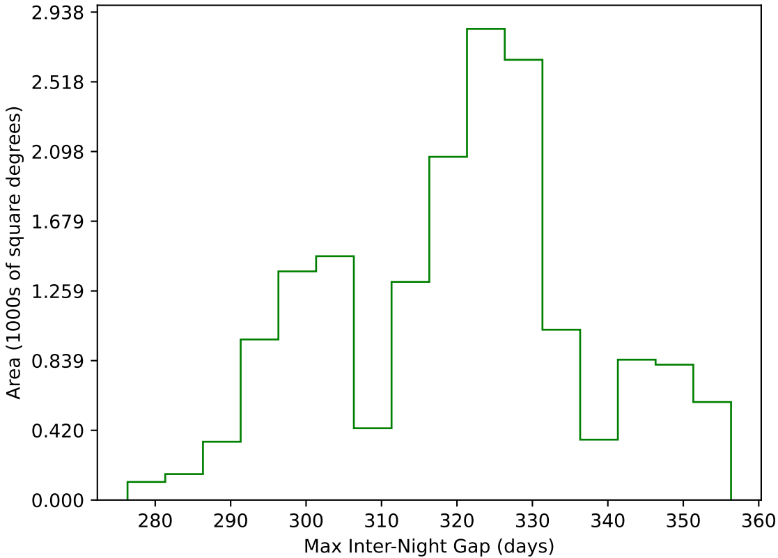
retro_baseline_v2.0_10yrs WFD g band: Max Inter-Night Gap
