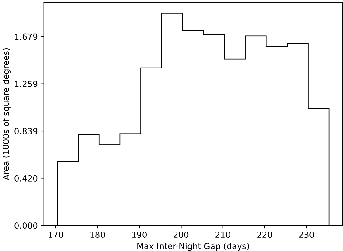
retro_baseline_v2.0_10yrs WFD all bands: Max Inter-Night Gap
