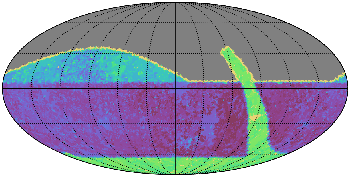
retro_baseline_v2.0_10yrs All sky z band: Max Inter-Night Gap
