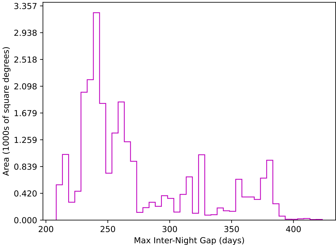
retro_baseline_v2.0_10yrs All sky z band: Max Inter-Night Gap
