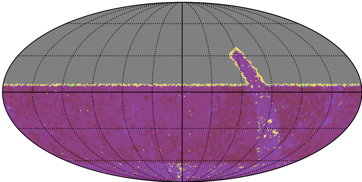
retro_baseline_v2.0_10yrs All sky u band: Max Inter-Night Gap
