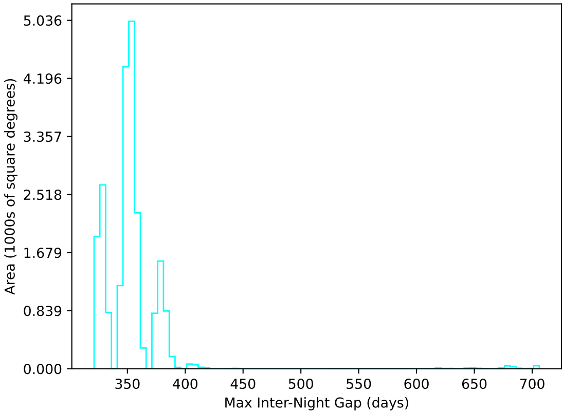
retro_baseline_v2.0_10yrs All sky u band: Max Inter-Night Gap
