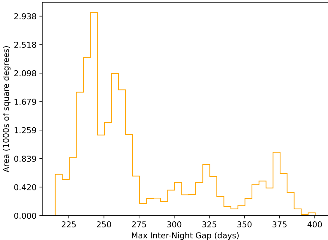
retro_baseline_v2.0_10yrs All sky r band: Max Inter-Night Gap
