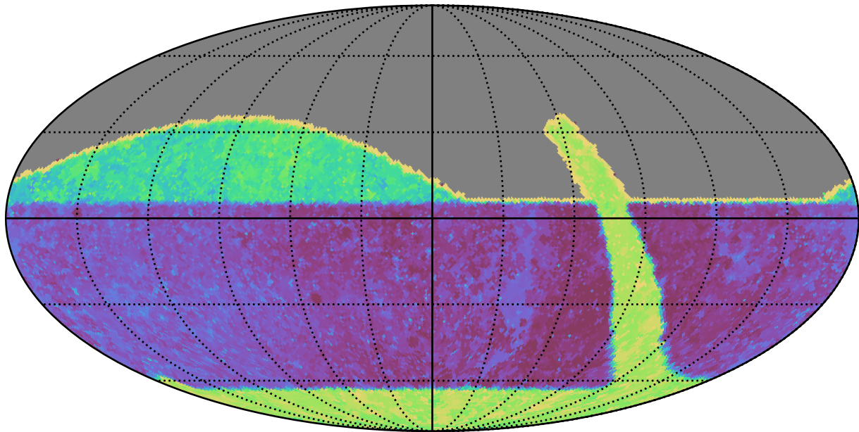
retro_baseline_v2.0_10yrs All sky i band: Max Inter-Night Gap
