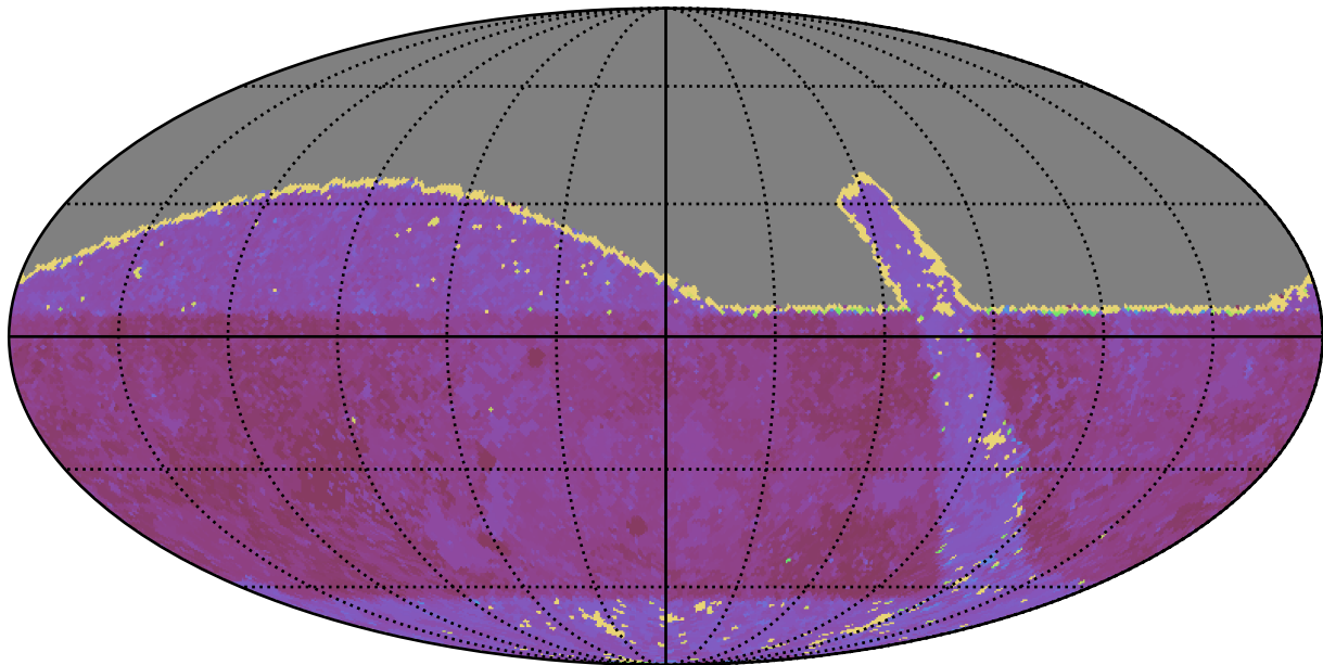
retro_baseline_v2.0_10yrs All sky g band: Max Inter-Night Gap
