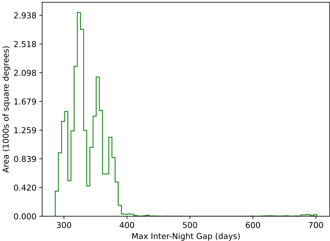
retro_baseline_v2.0_10yrs All sky g band: Max Inter-Night Gap
