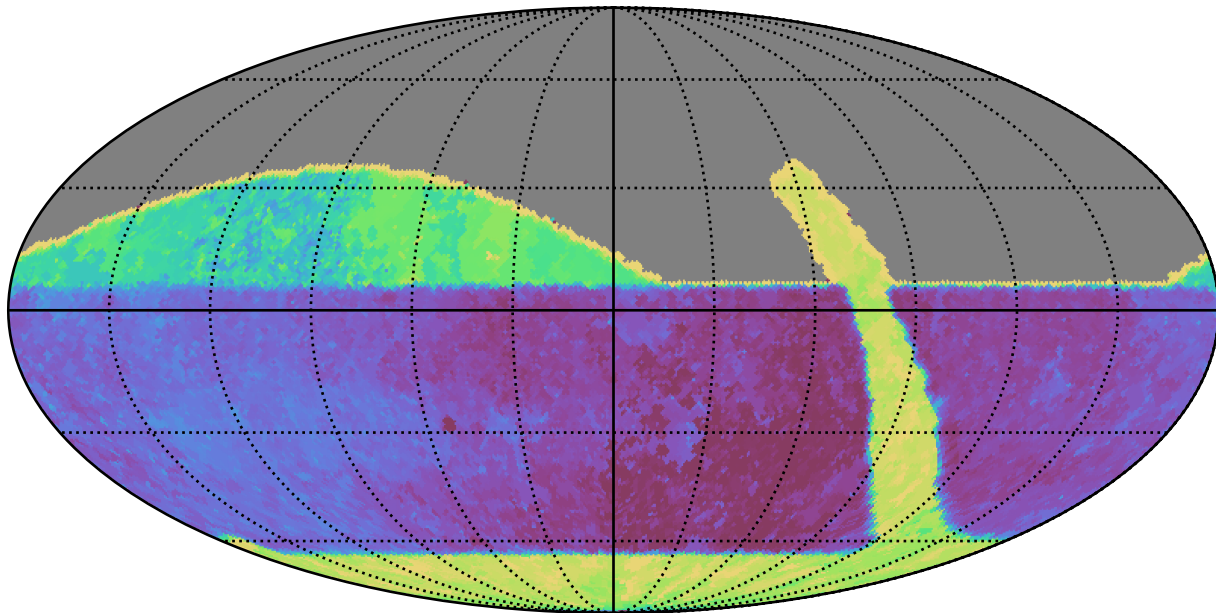
retro_baseline_v2.0_10yrs All sky all bands: Max Inter-Night Gap
