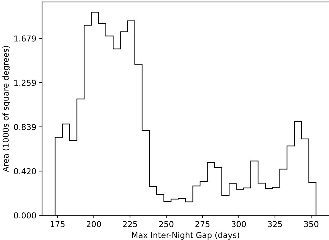
retro_baseline_v2.0_10yrs All sky all bands: Max Inter-Night Gap
