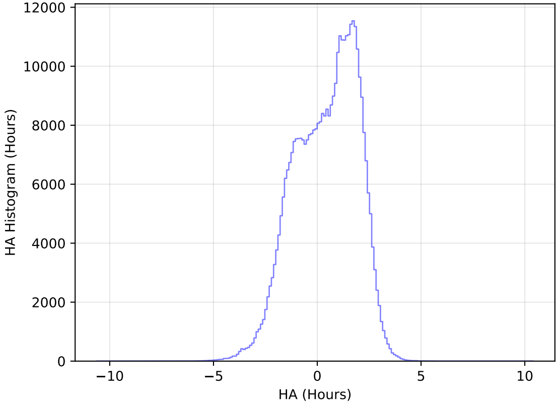
retro_baseline_v2.0_10yrs WFD z band: HA Histogram
