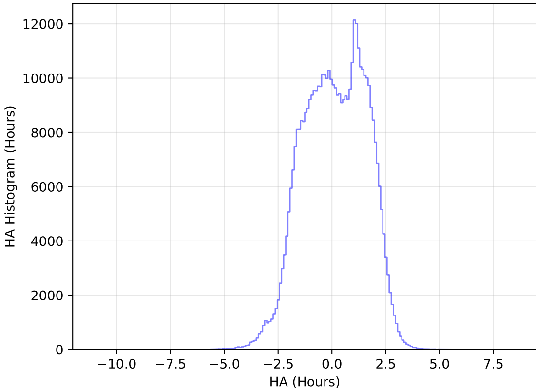
retro_baseline_v2.0_10yrs WFD r band: HA Histogram
