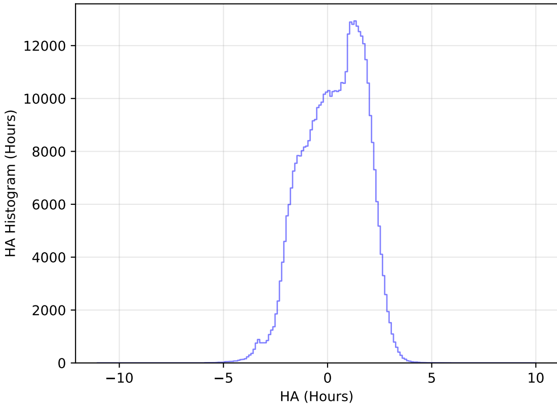
retro_baseline_v2.0_10yrs WFD i band: HA Histogram
