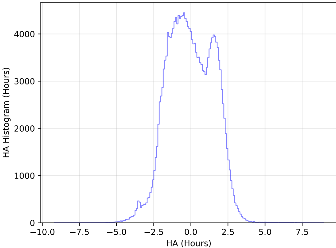
retro_baseline_v2.0_10yrs WFD g band: HA Histogram
