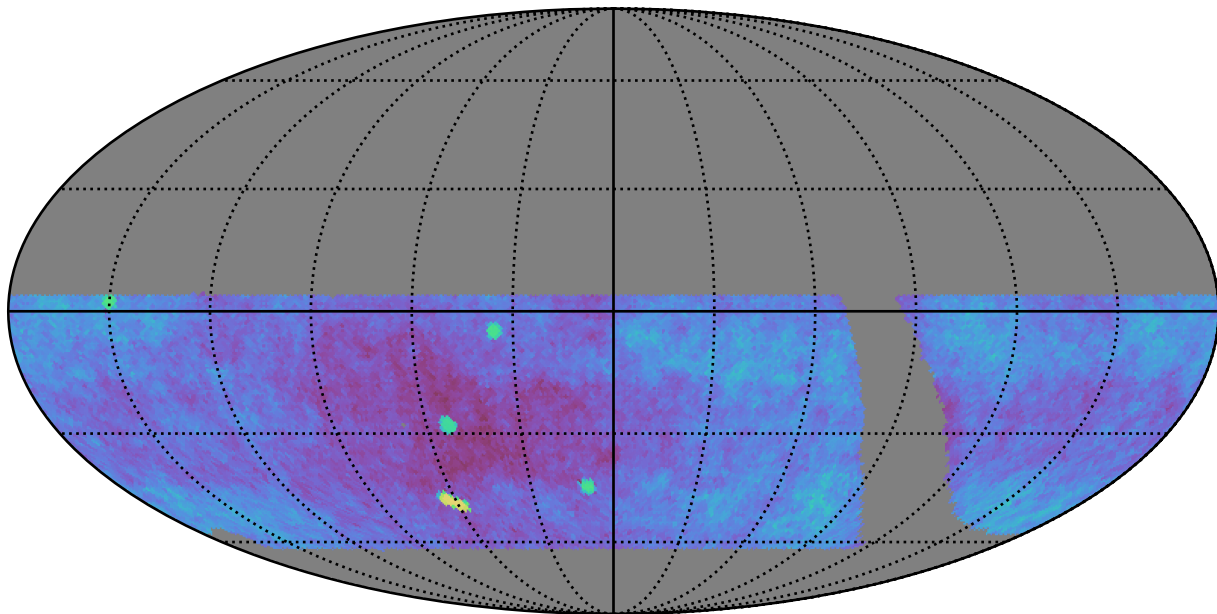
retro_baseline_v2.0_10yrs gri WFD: Fraction of visits in pairs (20-90 min)
